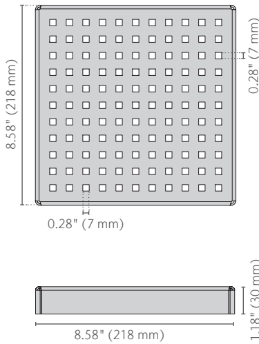
Quadrato Grate 10" LD 304/316L part no. 408097/408197
