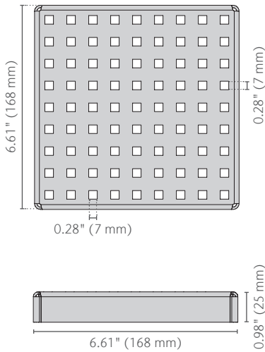
Quadrato Grate 8" LD 304/316L part no. 408092/408192
