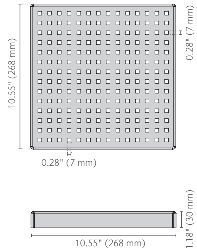
Quadrato Grate 12" LD 304/316L part no. 408036/408136
